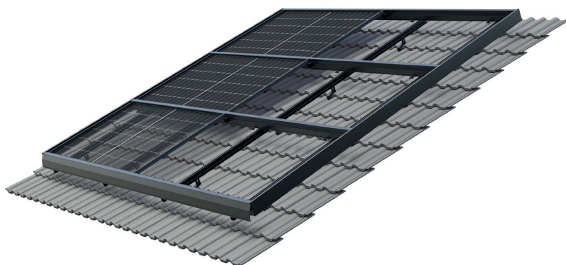
Roof-mounted S:FLEX Insertion System
